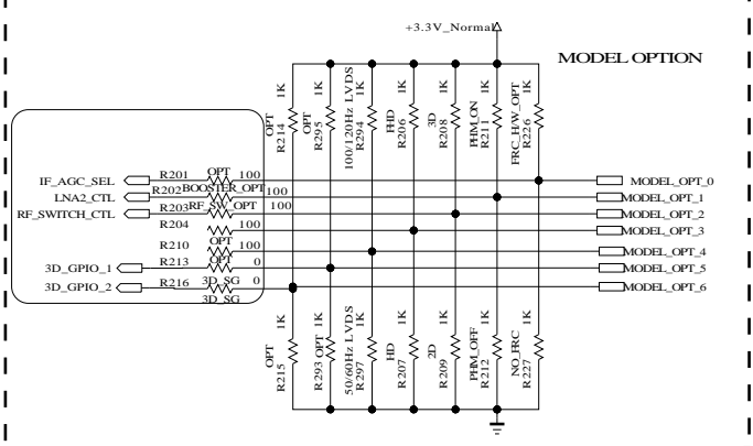
S7M-PLUS_DivX_MS10 IC101 GE107DC-RP [S7M+ DIVX/MS10]
