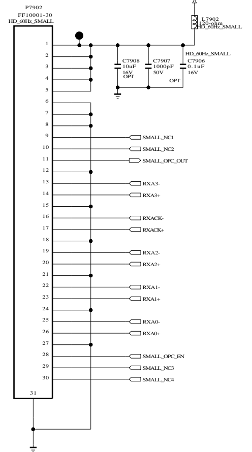
[30Pin LVDS Connector] (For HD 60Hz_Small)
