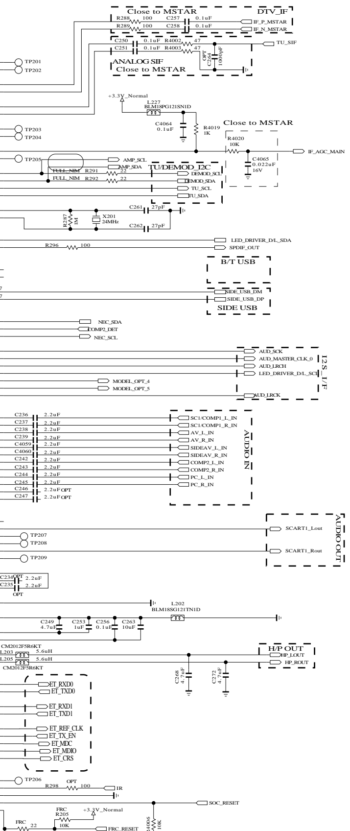
S7M-PLUS_DivX_MS10 IC101 GE107DC-RP [S7M+ DIVX/MS10]
