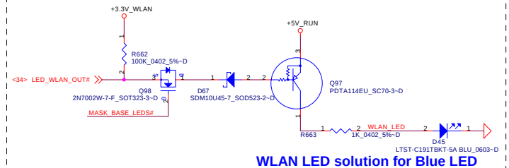
WLAN LED solution for Blue LED
