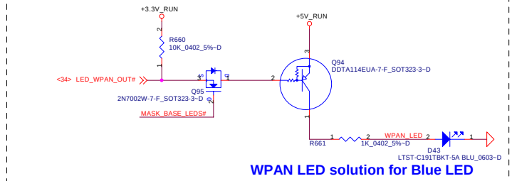
WPAN LED solution for Blue LED
