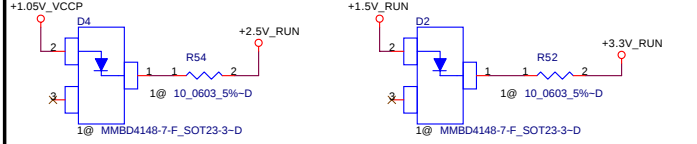
CRT DAC Voltage Follower Circuit - 700mV TV DAC Voltage Follower Circuit - 700mV
