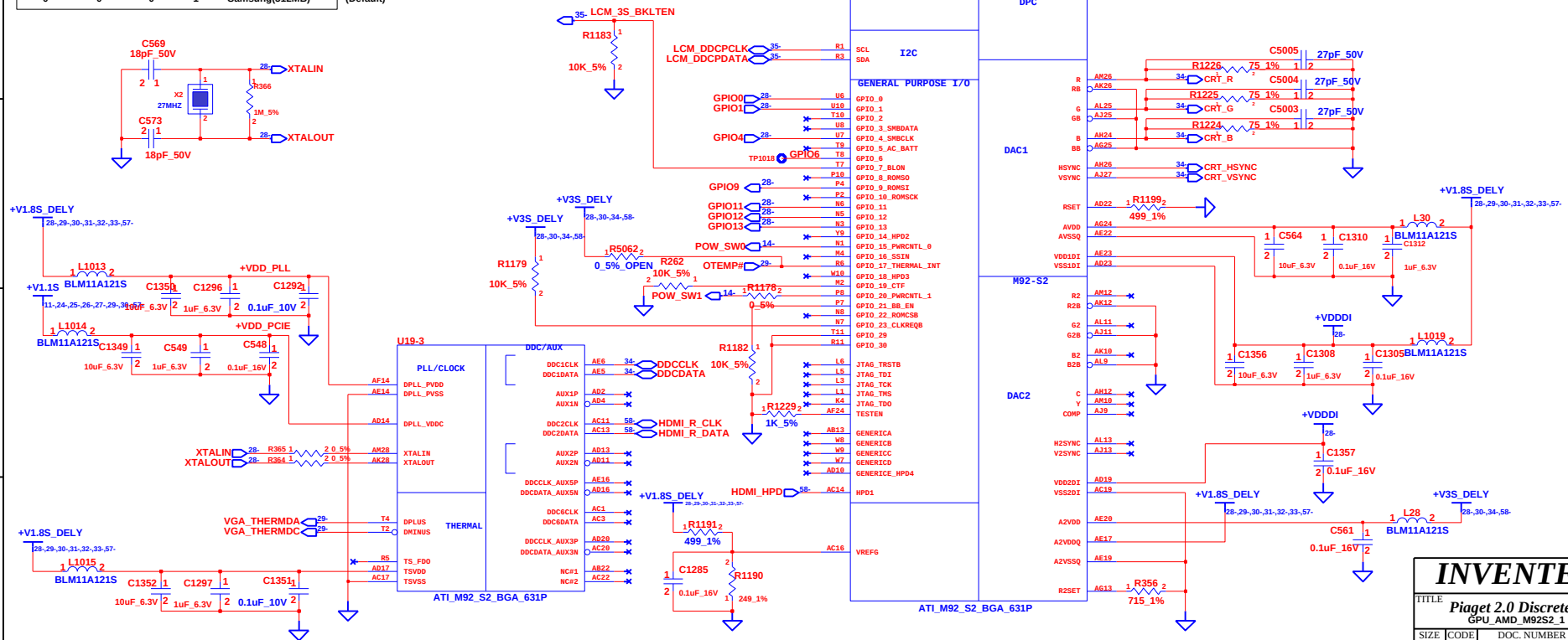
For DIS-GDDR2 MEM_ID3 MEM_ID2 MEM_ID1 MEM_ID0 vendor 0 0 1 1 hynix (512MB) 0 0 1 0 Qimonda(512M) 0 0 0 1 Samsung(512MB) (Default)
