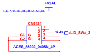
For LID SWITCH BOARD MB CONN
