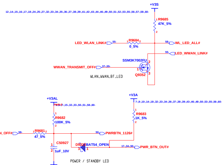
POWER / STANDBY LED
