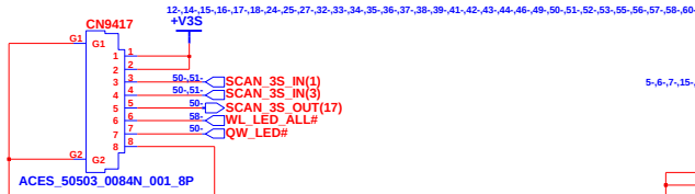
For QUICK LAUNCH BOARD MB CONN
