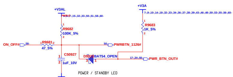
POWER / STANDBY LED
