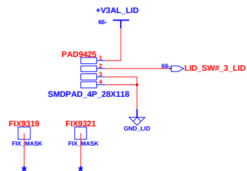
LID SWITCH Reference Number 9200-9299
