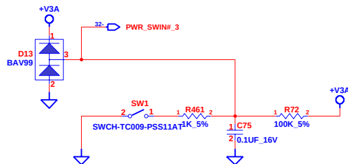
PWR SWITCH
