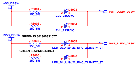
LED & SWITCH
