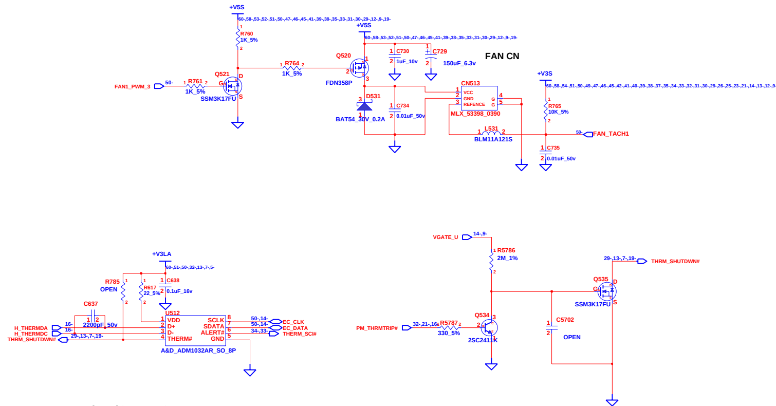
Thermal Sensor For CPU
