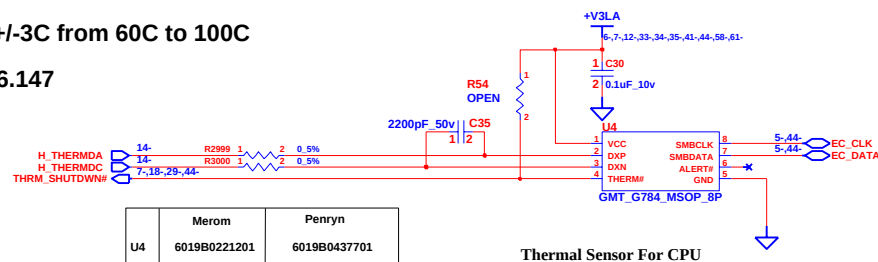
Thermal Sensor For CPU
