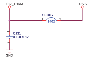
Thermal Sensor Power Supply
